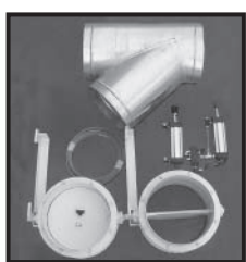
Blast Gate Assembly 14" & 16" Double
